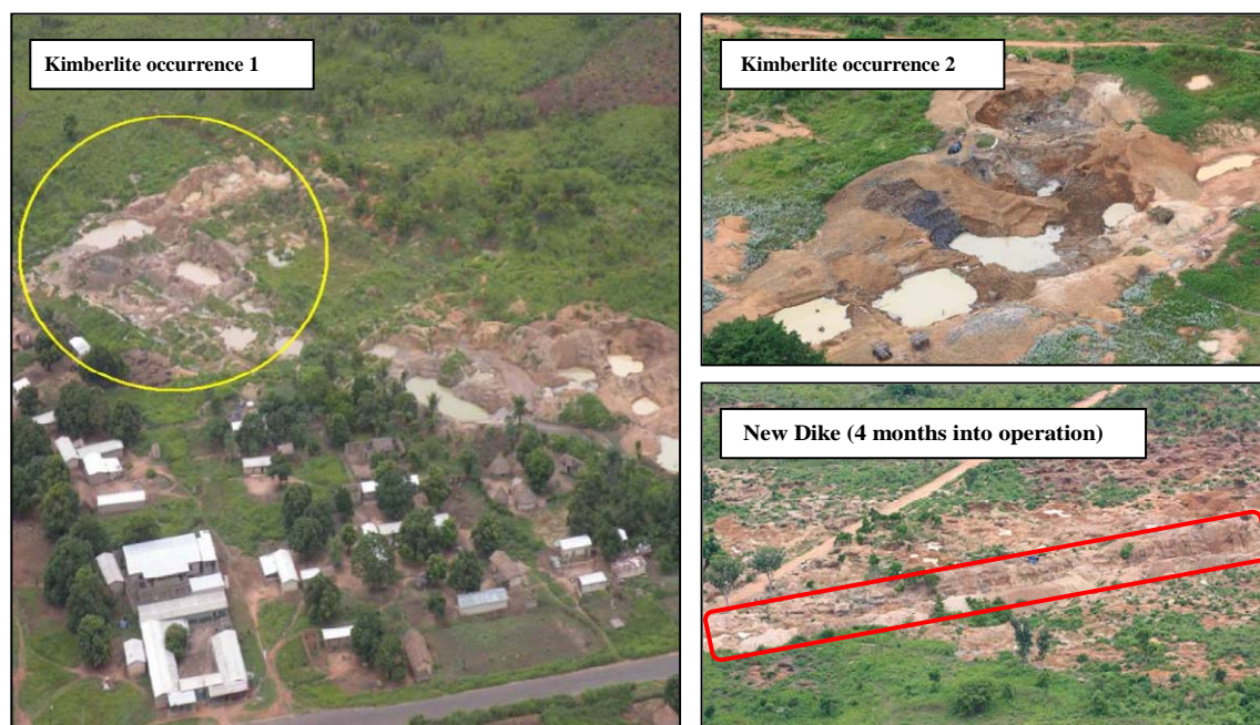
Figure XIV Kimberlite occurrences, Séguéla, May 2009
