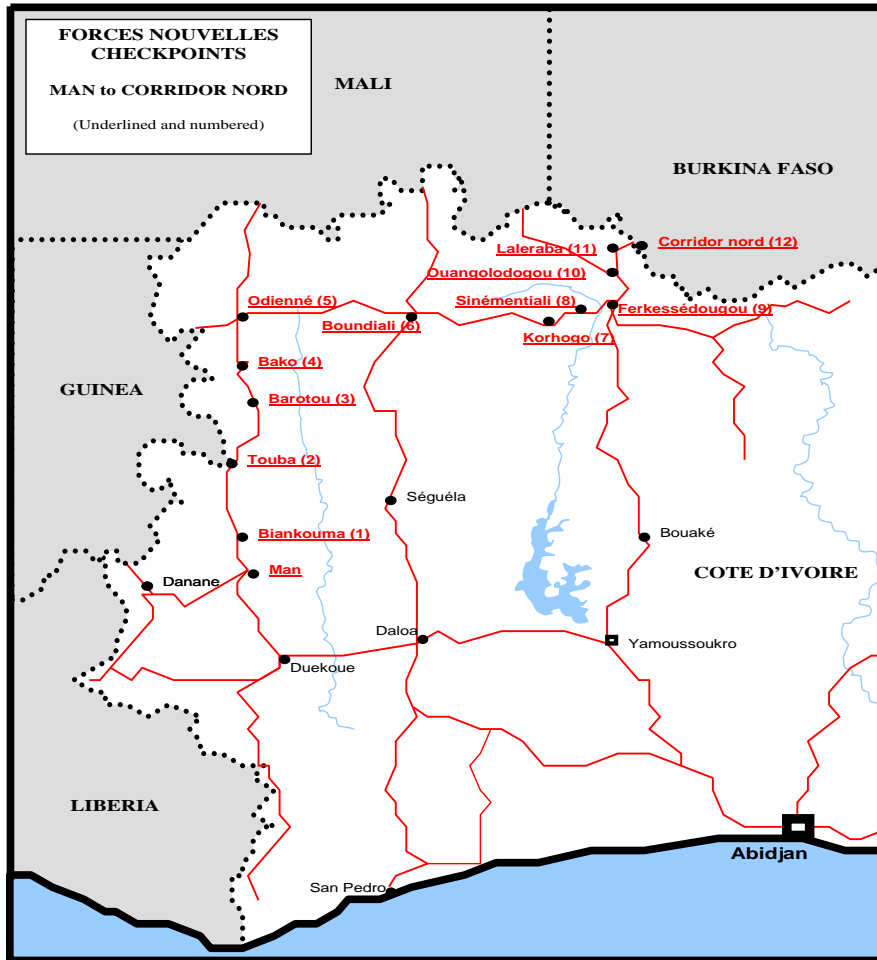
Figure X Forces nouvelles checkpoints on route from Man to Corridor Nord
